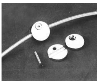
FRONT BRAKE LINE CLAMP (DISC) BLC001
